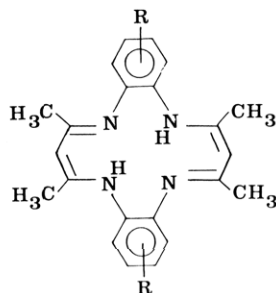
Figure 1. [\text{H}_2\text{Me}_4(\text{RBzo})_2[14]\text{tetraeneN}_4] .
