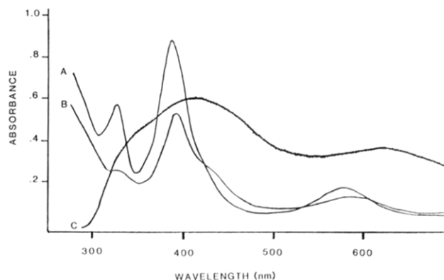
Figure 6. Visible spectra of the monomer, dimer, and polymer derived from [\text{Ni}(\text{Me}_4\text{BzO}_2[14]\text{tetraeneN}_4)] : (A) absorption spectrum, 3 \times 10^{-5} M [\text{Ni}(\text{Me}_4\text{BzO}_2[14]\text{tetraeneN}_4)] in DMF; (B) 2 \times 10^{-5} M [\text{Ni}(\text{Me}_4\text{BzO}_2[14]\text{tetraeneN}_4)]_2(\text{ClO}_4)_2 in DMF; (C) transmission spectrum, [\text{Ni}(\text{Me}_4\text{BzO}_2[14]\text{tetraeneN}_4)]_n on a \text{SnO}_2 plate. The absorbance scale for the latter spectrum is arbitrary.
