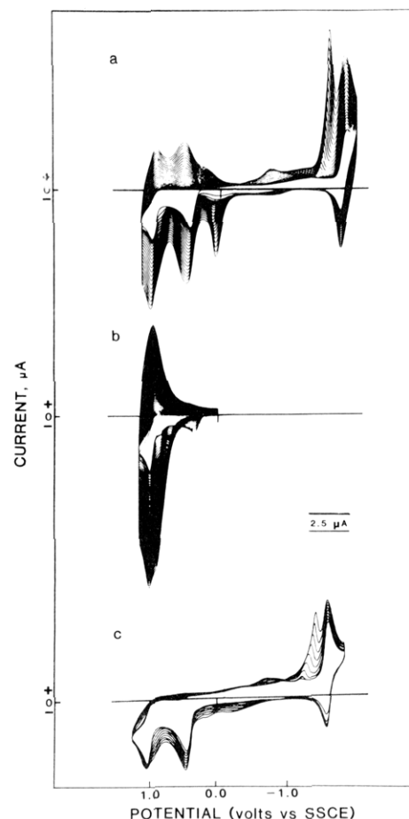
Figure 2. Cyclic voltammograms of film growth on Pt electrodes in acetonitrile solutions containing 0.1 M TEAP and 1.0 \times 10^{-3} M complex: (a) [\text{Ni}(\text{Me}_4\text{Bzo}_2[14]\text{tetraeneN}_4)] , scan range +1.4 to -1.9 V vs. SSCE; (b) [\text{Ni}(\text{Me}_4\text{Bzo}_2[14]\text{tetraeneN}_4)] , scan range 0 to 1.4 V vs. SSCE; (c) [\text{Ni}(\text{Me}_4(\text{CH}_3\text{CO}_2\text{Bzo})_2[14]\text{tetraeneN}_4)] , scan range +1.4 to -1.9 V vs. SSCE. The scan rate was 200 mV/s.
